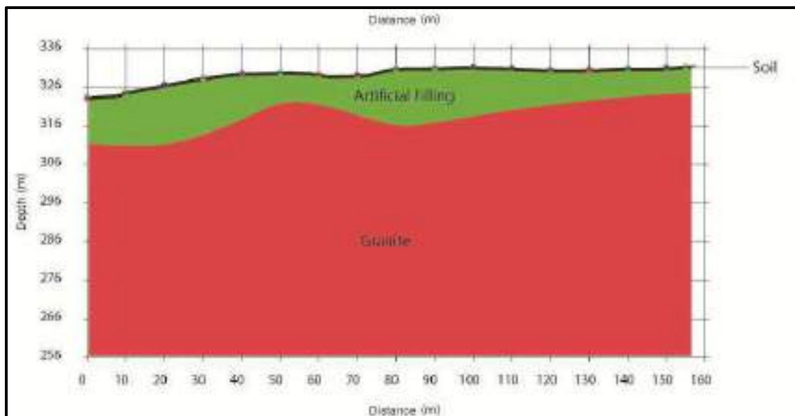
Figura 2-3. Geophysical Profile P1.
